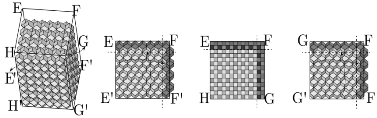
Figure 2. for the online cube sphere, the darker rhombic dodecahedral cells are lost by subdividing a q - bin(i, p) into a hexagon. The boundary of q - bin(i, p) is a thick line. The lines and boundaries of the area between the dashed lines are considered missing.
