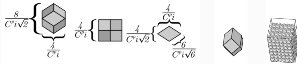
Figure 1. specific numerical relationship of cell units (left); fill a q-bin(i, p) (right)
